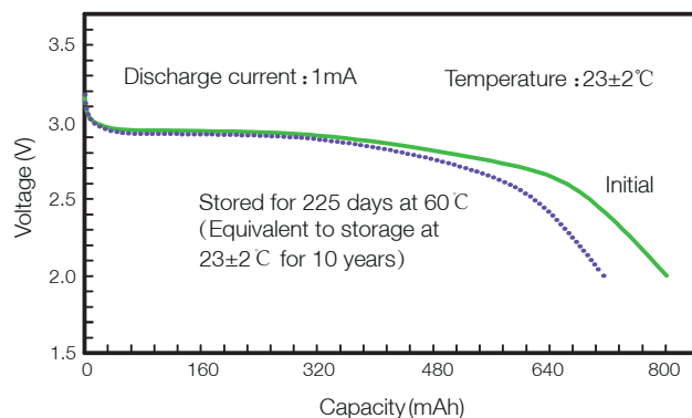
3. Storage characteristics
