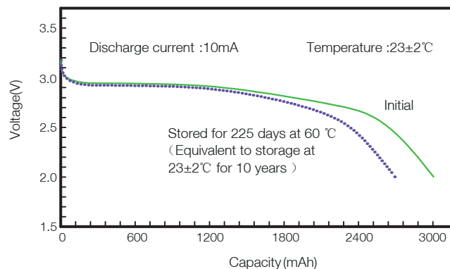
3. Storage characteristics
