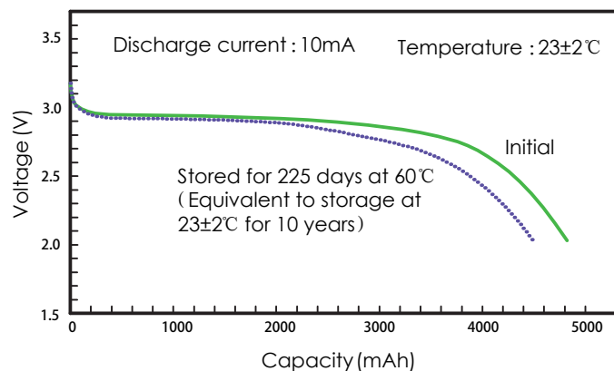
3. Storage characteristics
