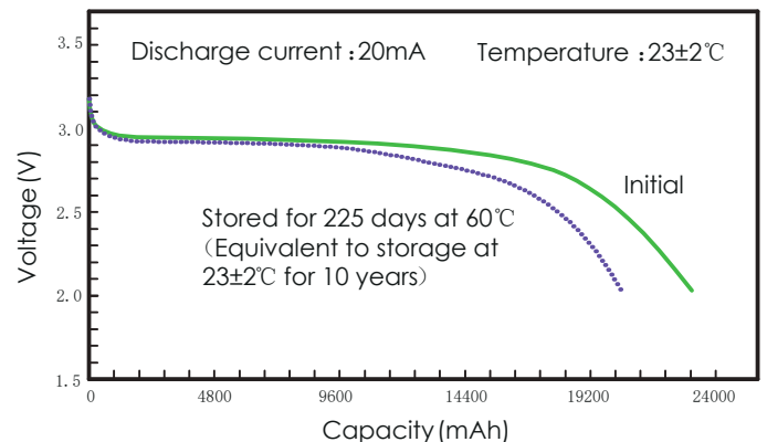
3. Storage characteristics
