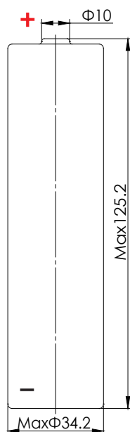
Dimensions in mm
