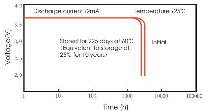
3. Storage characteristics
